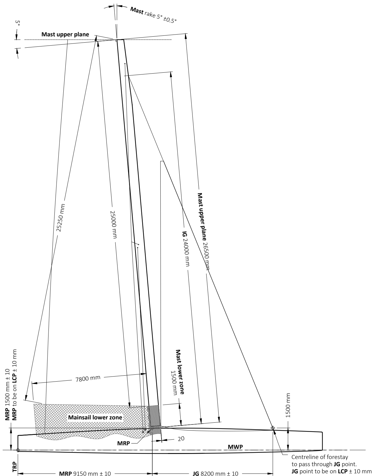
Figure 17.1: Sail Plan
